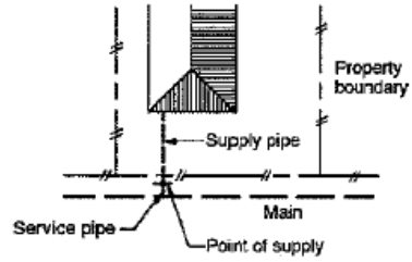
Type 2: Point of supply outside property
