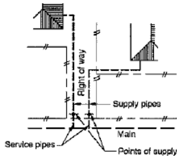
Type 1: Point of supply inside boundary
