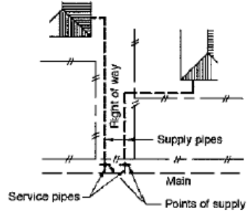
Type 2: Point of supply outside property
