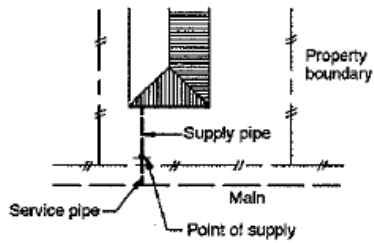
Type 1: Point of supply inside boundary
