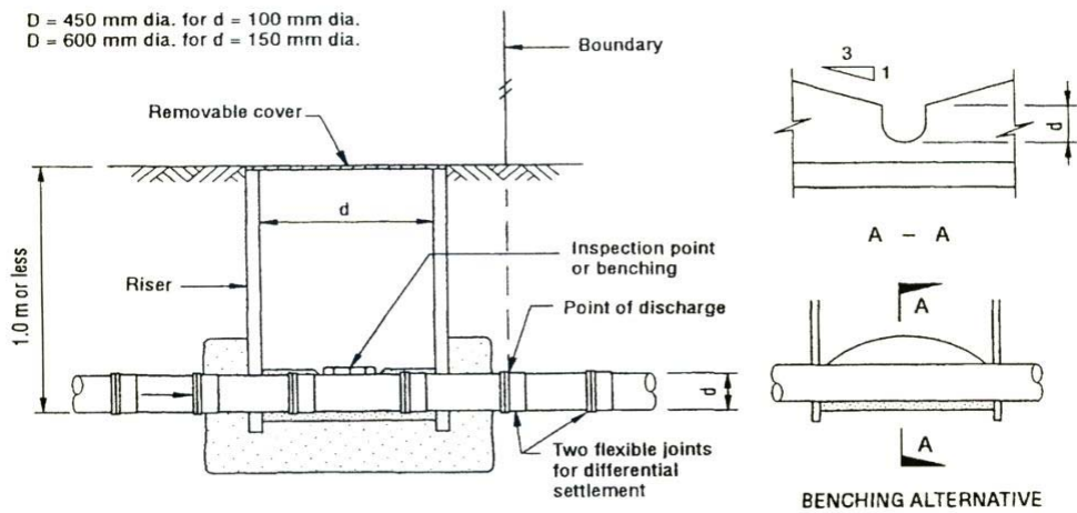
'CONTROLLED' TRADE WASTE DISCHARGES, NOT GREATER THAN 1.0 METRE DEEP
