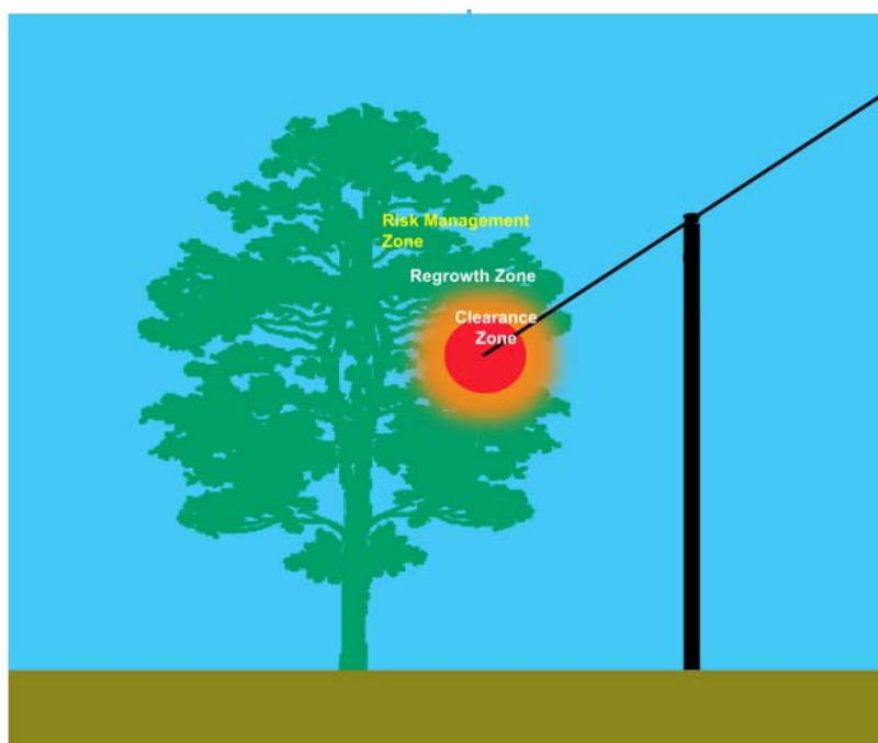
Figure 2 – Clearance Profile – Low Voltage ABC and Insulated Service Cable
