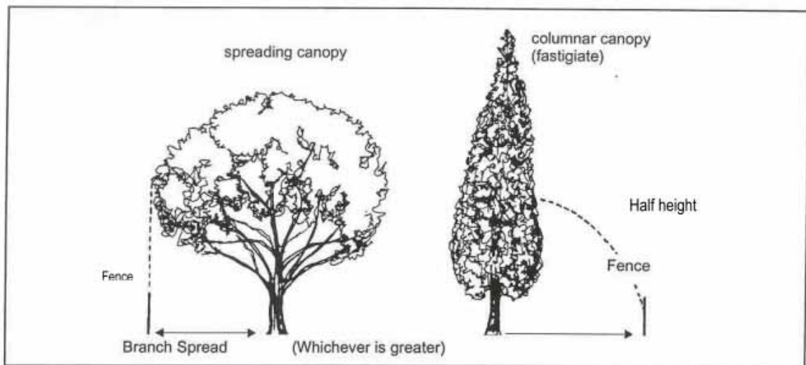
Figure 11 Dimensions for locating perimeter fencing
