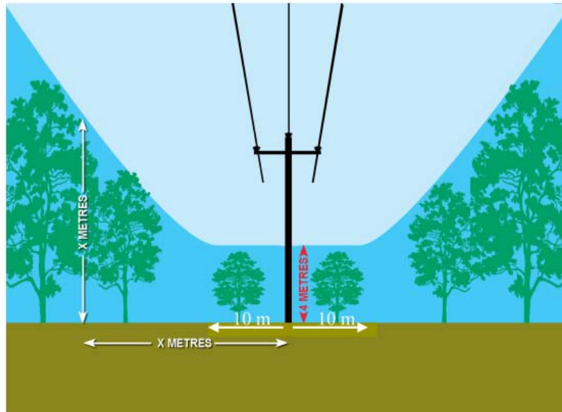
Figure 3. Rural and Sub Transmission - Bare Wire Conductor Systems Corridor Profile
